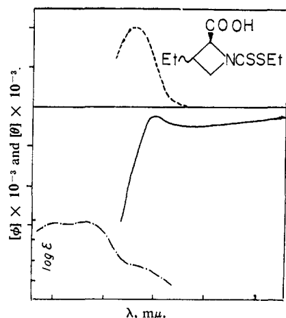
Figure 7. ORD (—), CD (---), and uv (- - -) curves of N -dithiocarboxy-( S )-dihydropolyoximic acid ( 23 ) in methanol.
