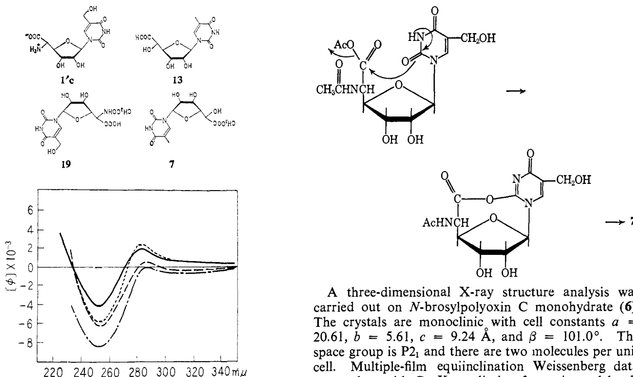
Figure 3. ORD curves of polyoxin C (1'c) (—), deaminodeoxy-polyoxin C (8) (---), methyl deaminodeoxypolyoxinate (19) (-.-), and N -acetylpolyoxin C (7) (.....).
